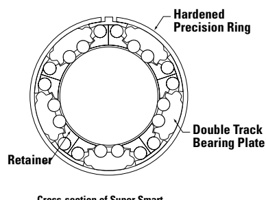
Figure 1 Cross-section of Super Smart Ball Bushing Bearing
